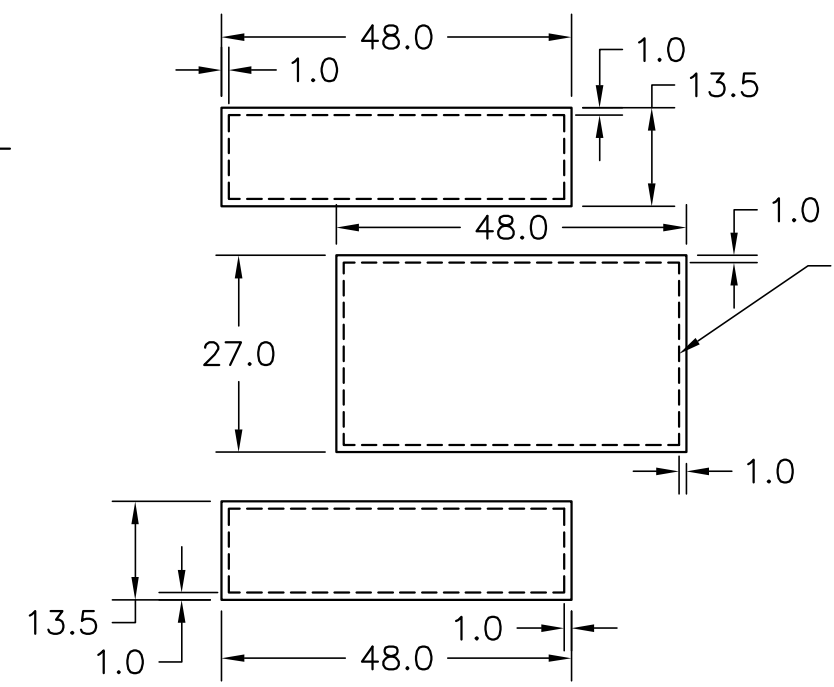
DETAIL AA SCALE: NTS
